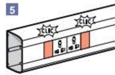
Snap on the finishing piece
