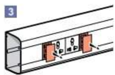
Disengage the finishing piece
