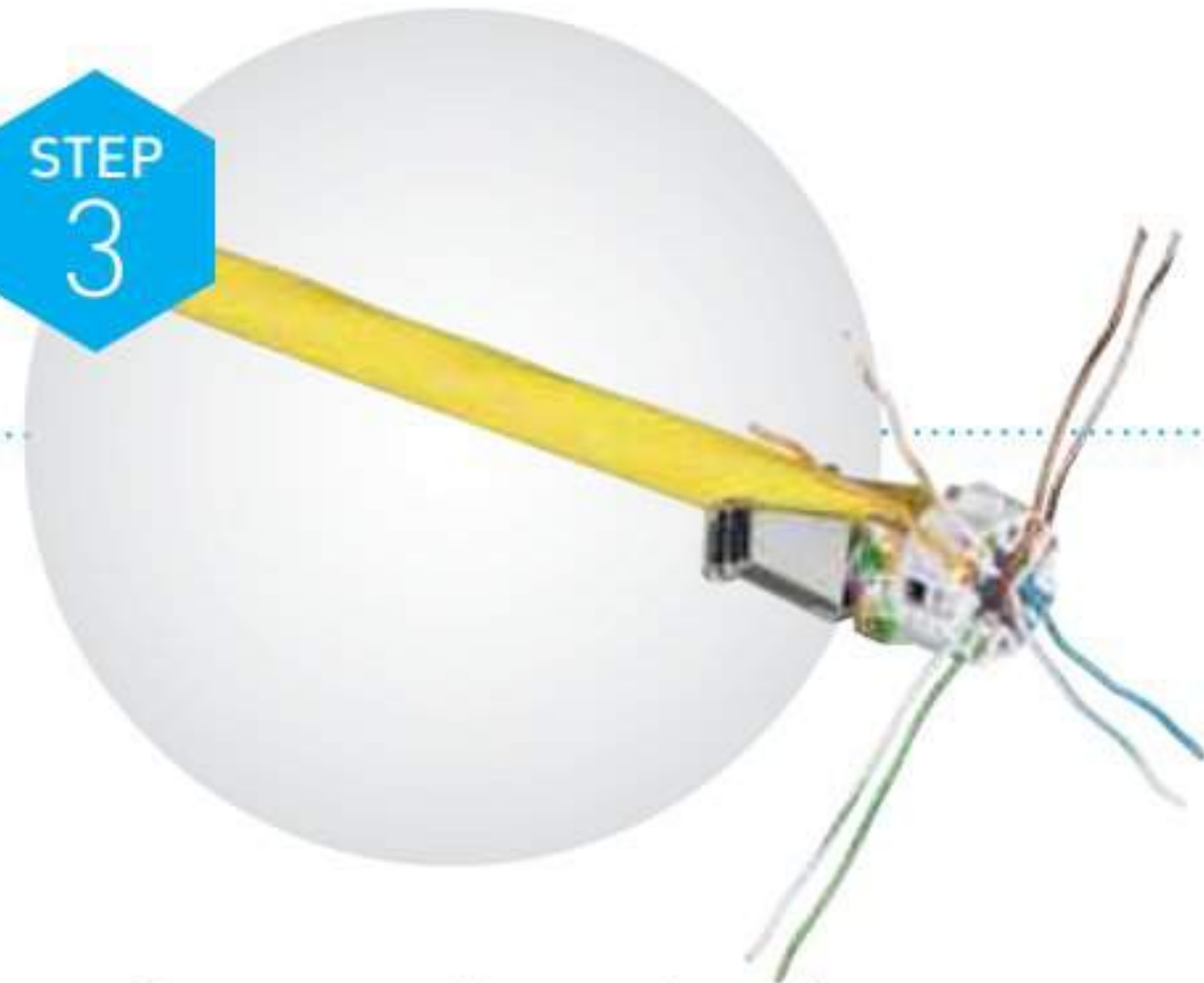
Separate and insert the pairs
